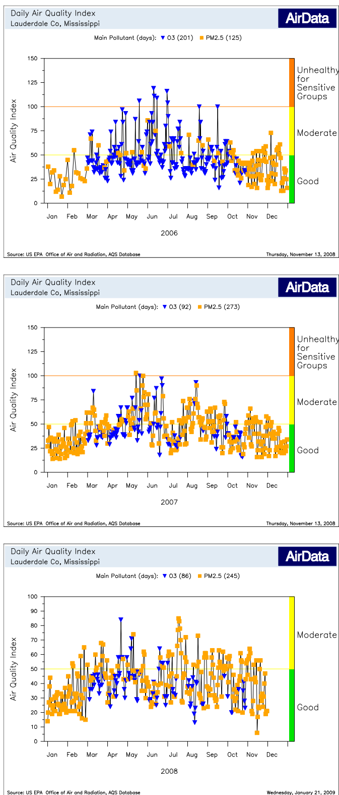
Figure 3.3-3. AQI Charts for Lauderdale County—2006 through 2008
