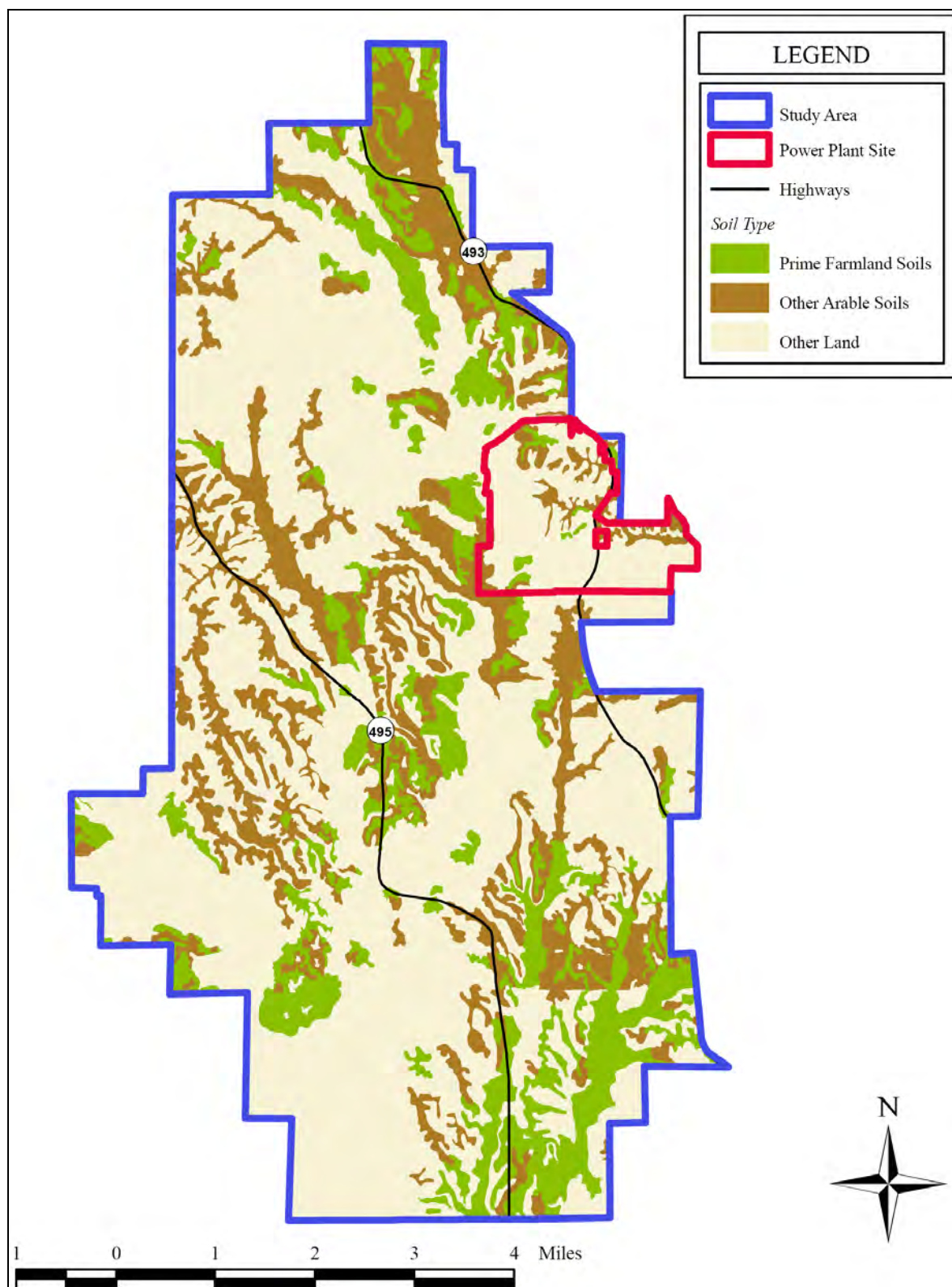
Figure 3.5-2. Geographic Locations of Soil Map Units
