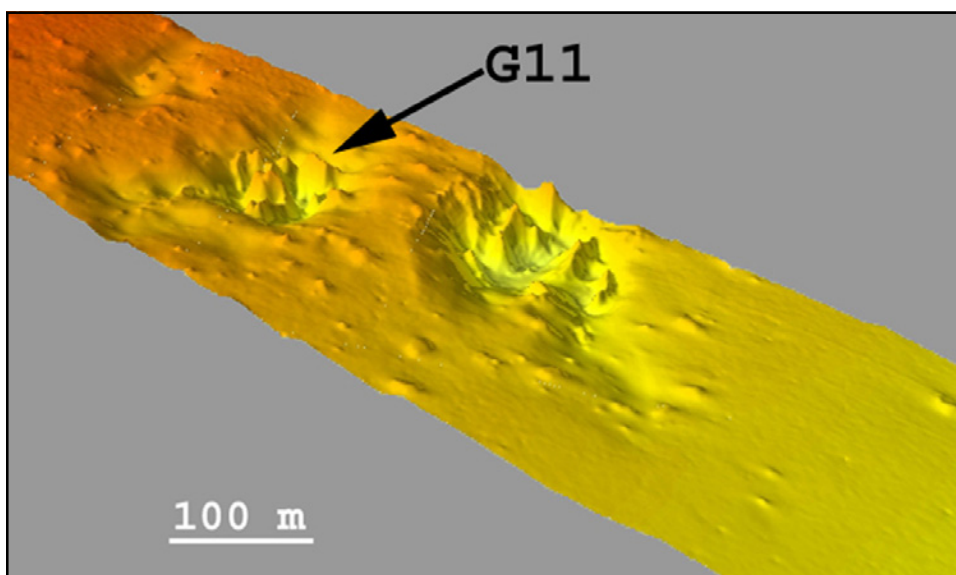
Echosound image of the Nyegga site with vertical scale enhanced by a factor of three. The pockmark named “G11” has a diameter of about 150 m and is the primary study location.
