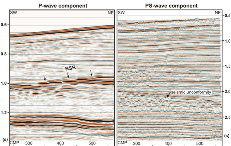
Stacked sections of P-wave and the PS-wave component of the OBC line, which has a length of approximately 4 km. Note the difference in time axis. The inline component has been linearly stretched in time to match the P wave data based on a horizon, which occurs just below a sedimentary layer with chaotic internal texture labeled "seismic unconformity."
